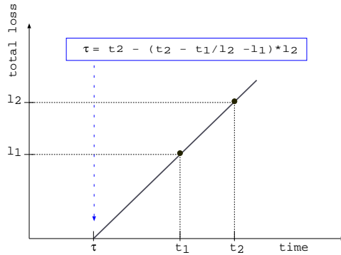
Figure 6: Determining the buffer size.
