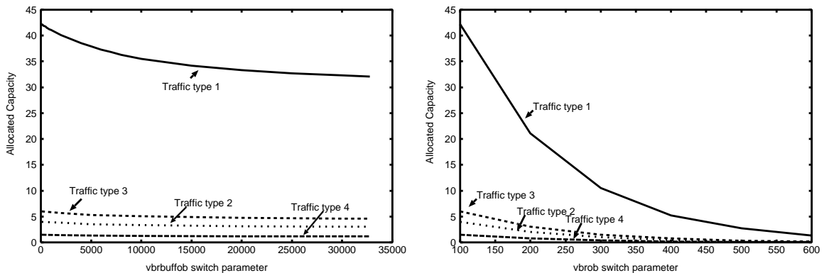
Figure 3: The allocated capacity versus the overbooking parameters of the Fore-Systems ASX-1000 ATM switch
