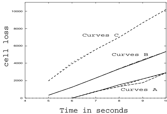
Figure 8: Number of lost cells for each PVC as a function of time: traffic with different UPC contracts. (The traffic policing is disabled at all ports of the ATM switch.)
