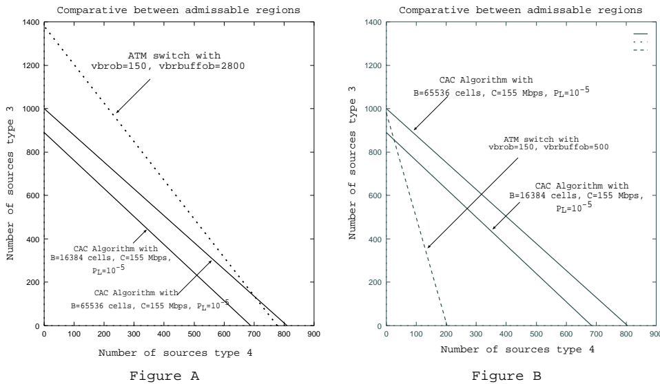
Figure 5: Effective capacity: heterogeneous sources.
