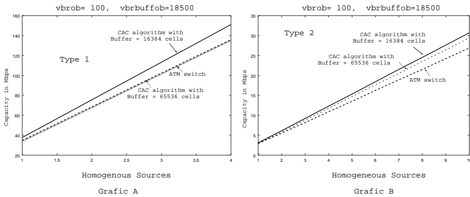
Figure 4: Effective capacity: homogeneous sources.
