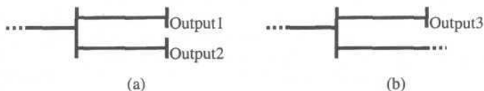
Figure 12 - Different UCM And-fork constructions
