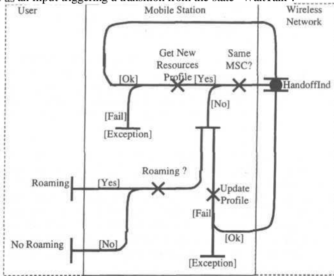
Figure 19 - Handoff use case map
