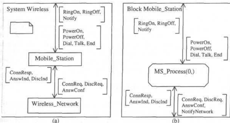
Figure 5 - A sample SDL architectural system
