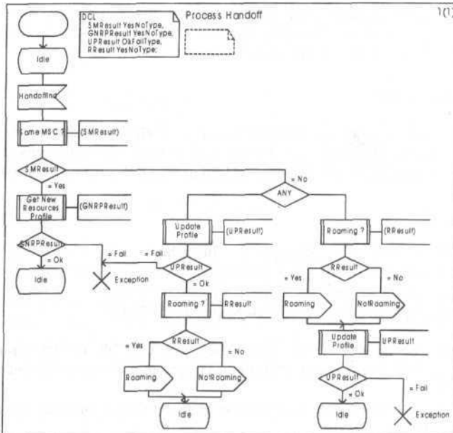
Figure 20 - Handoff SDL behaviour
