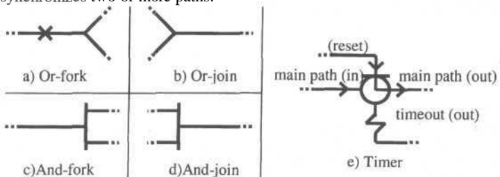
Figure 3 - Different Use Case Map Constructions
