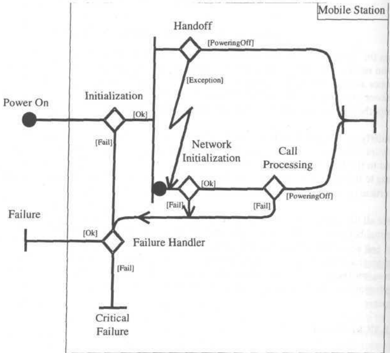
Figure 9 - High-Level Behaviour UCM model
