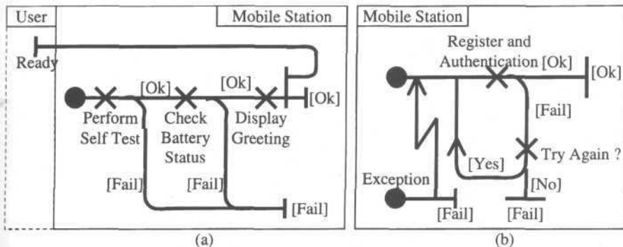
Figure 15 - The Initialization and Network Initialization UCMs
