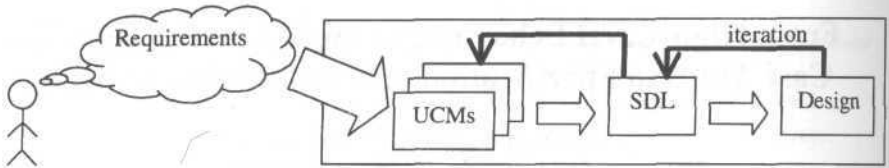
Figure 1 – From Use Case Maps to SDL
