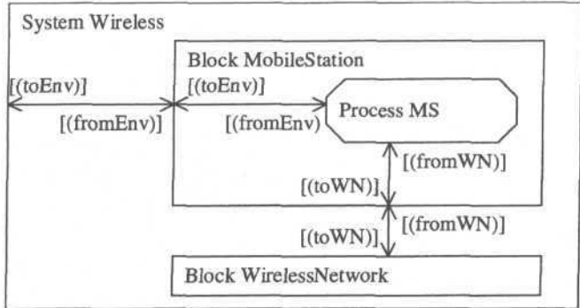
Figure 10 - The SDL overview of the architecture for a Mobile Station
