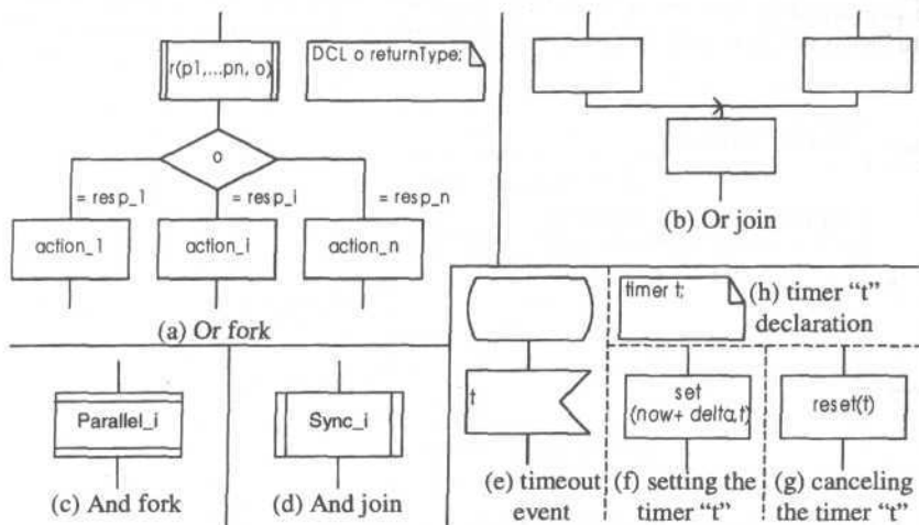
Figure 11 - SDL common structures for representing UCMs
