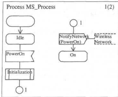
Figure 6 - A sample SDL process chart
