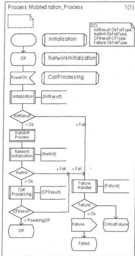
Figure 14 - The SDL behaviour for the root UCM
