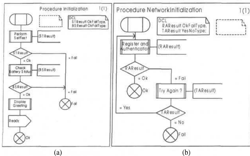
Figure 16 • The SDL behaviour for the Initialization procedures maps
