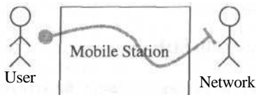
Figure 8 - Final UCM architecture
