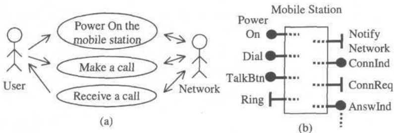
Figure 7 - Use Case Diagram and Use Case Maps
