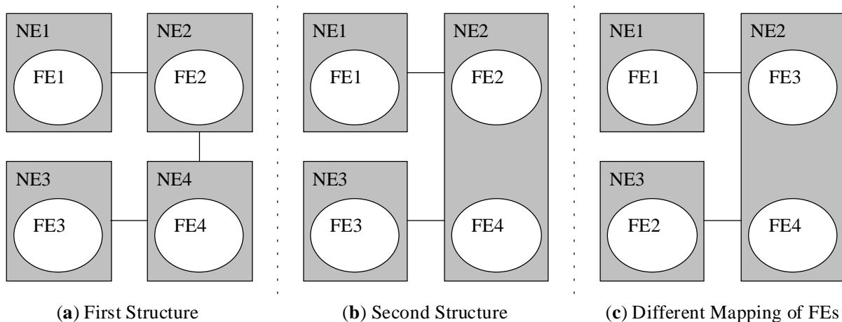
Figure 4 Different Bindings of Functional Entities to Network Entities
