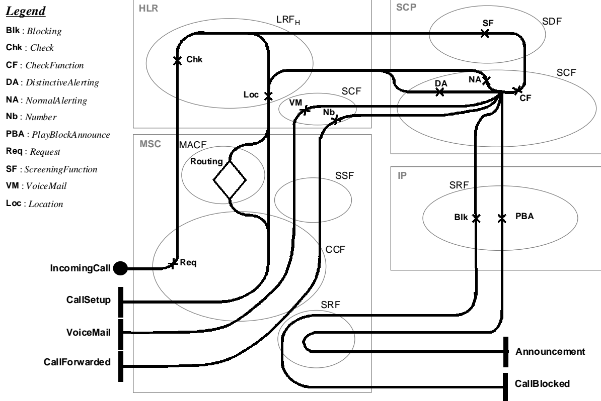
Figure 11 UCM Plugin for the ICS Stub
