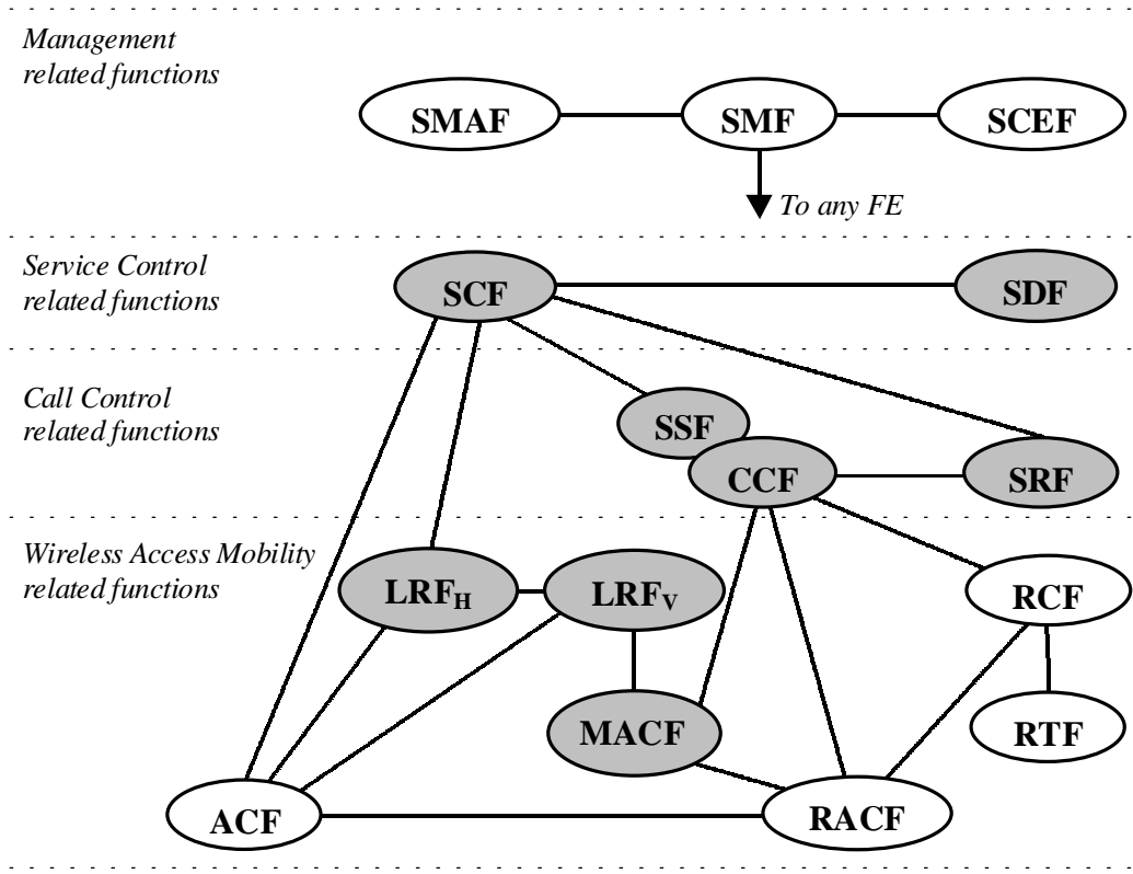
Figure 6 Wireless Distributed Functional Model (adapted from Figure 1 of IS-41.7-WIN [18])
